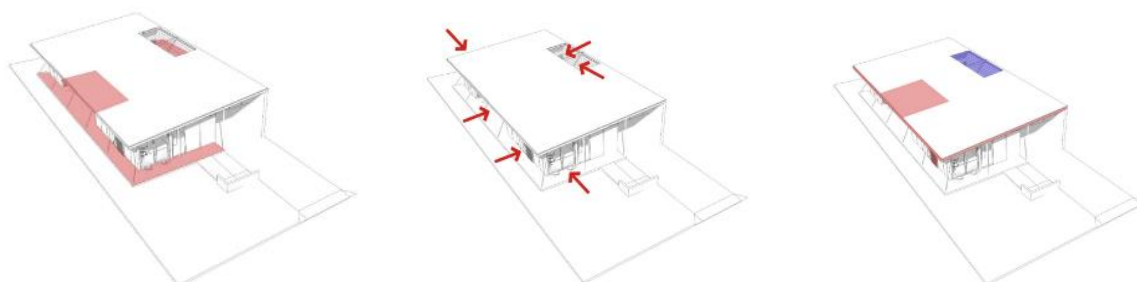
Concept sketches of key principles - northern exposure for pleasant outdoor spaces, various features used to shade windows from the summer sun and courtyards added for maximising solar access.
