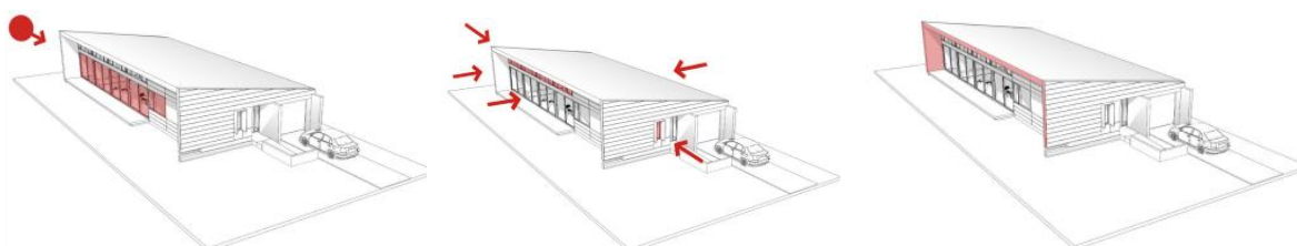
Concept sketches of key principles – design shaped to maximise northern exposure and preserve pleasant outdoor spaces, and various features used to shade windows from the summer sun.
